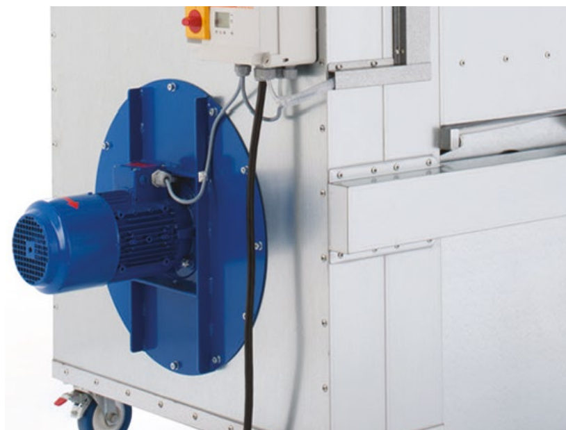
Illustration above: Vacumobil VT 160 with 2.2 kW energy-saving motor (IE3)
